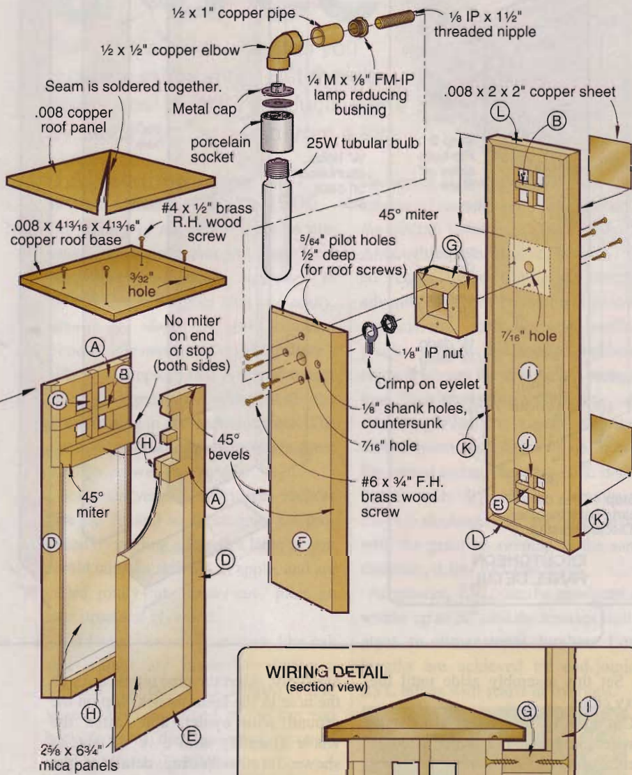
EXPLODED VIEW
